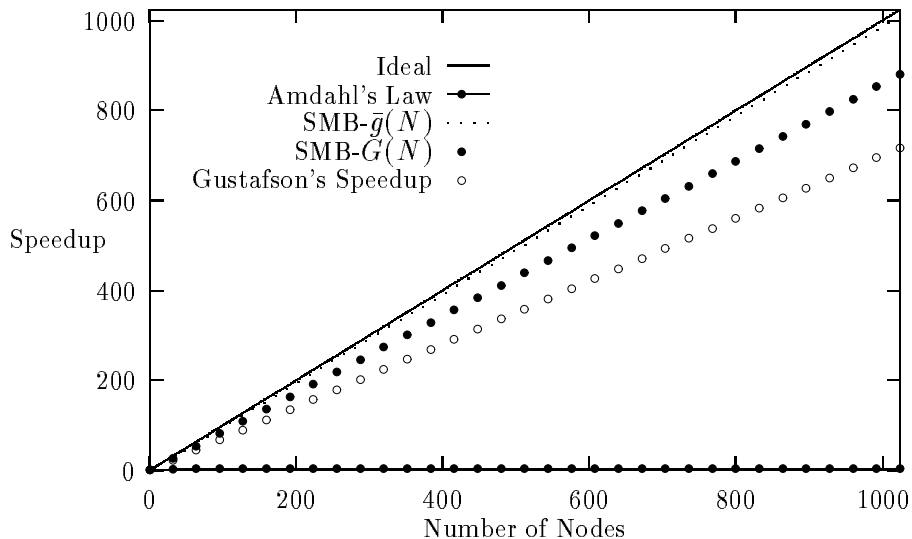
Figure 5. Amdahl's law, Gustafson's speedup, and SMB speedup for k = 0.3 .
