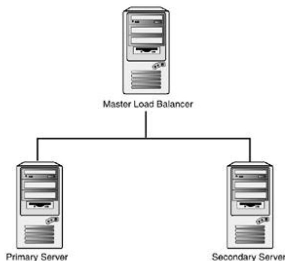
Figure 1.2. Load balancing 101.
